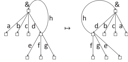
Figure 9. \mathbf{u-sbl}(\text{swap-hd-tl})
