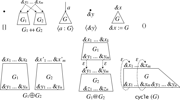
Figure 3. Graph Constructors
