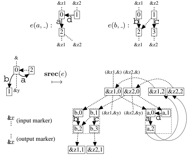
Figure 7. Bulk Semantics of Structural Recursion
