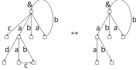
Figure 11. left_a_path
