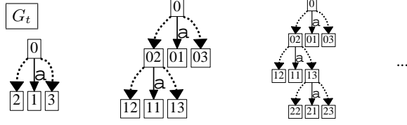
Figure 12. Branch with Any Countable Linear Order
