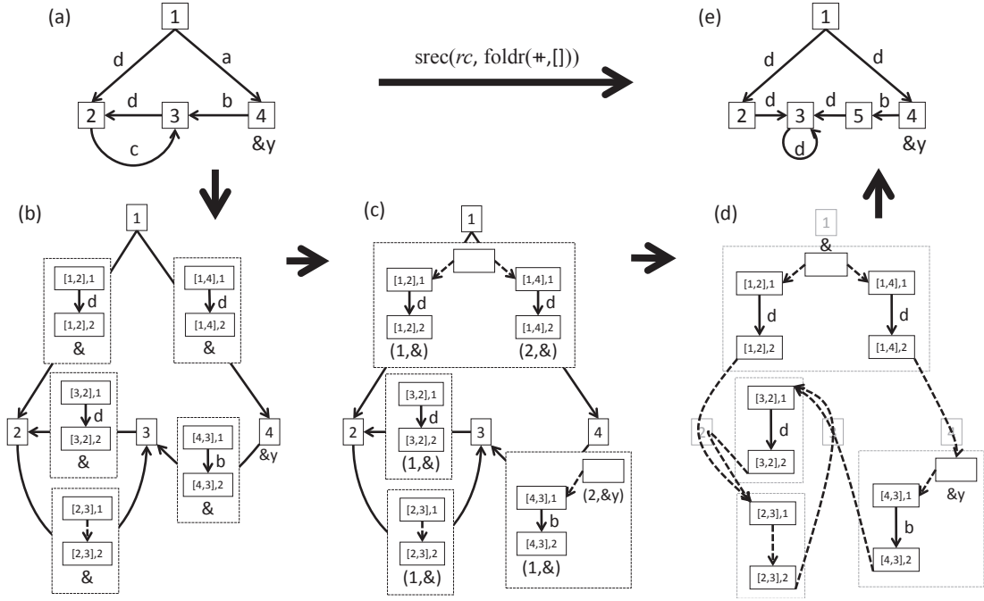
Figure 10. Bulk Semantics of Structural Recursion: An Example of \text{srec}(rc, \text{foldr}(\#, []))
