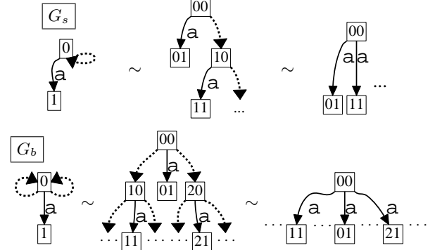
Figure 6. Graphs with Stream Branching and with Dense Branching
