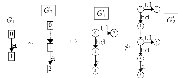
Figure 1. An Example of Unsound Encoding
